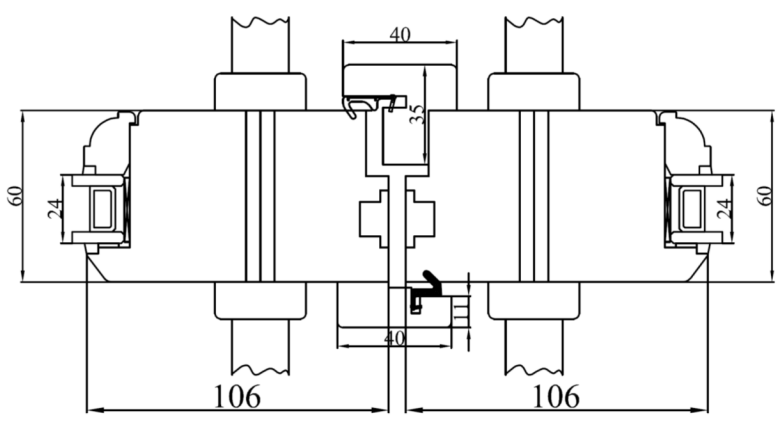
Section C-C
